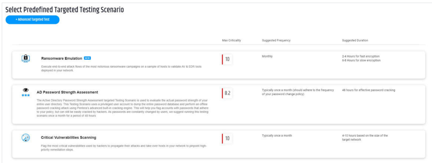
Figure 7. Predefined Scenarios Available in Pentera's Targeted Testing
